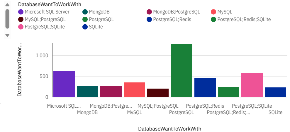
column chart showing Top 10 Database Want To Work With.
